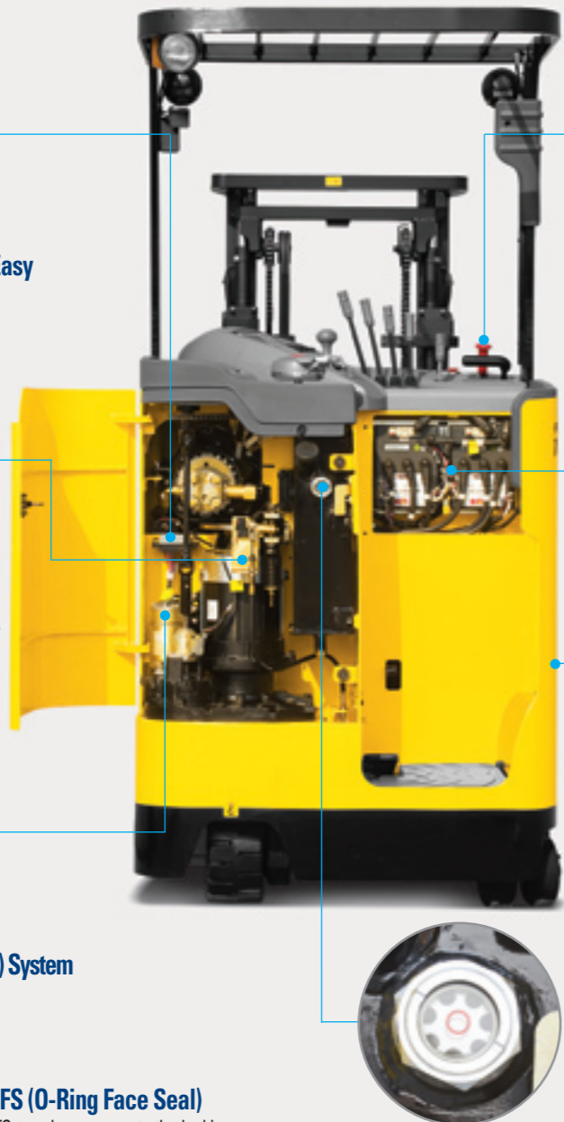
Hydraulic Oil Level Gauge
